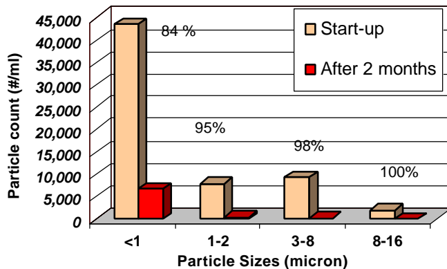
Cooling Tower Loop Particle Count Sartomer Chemicals Westchester, PA after 2 month period
